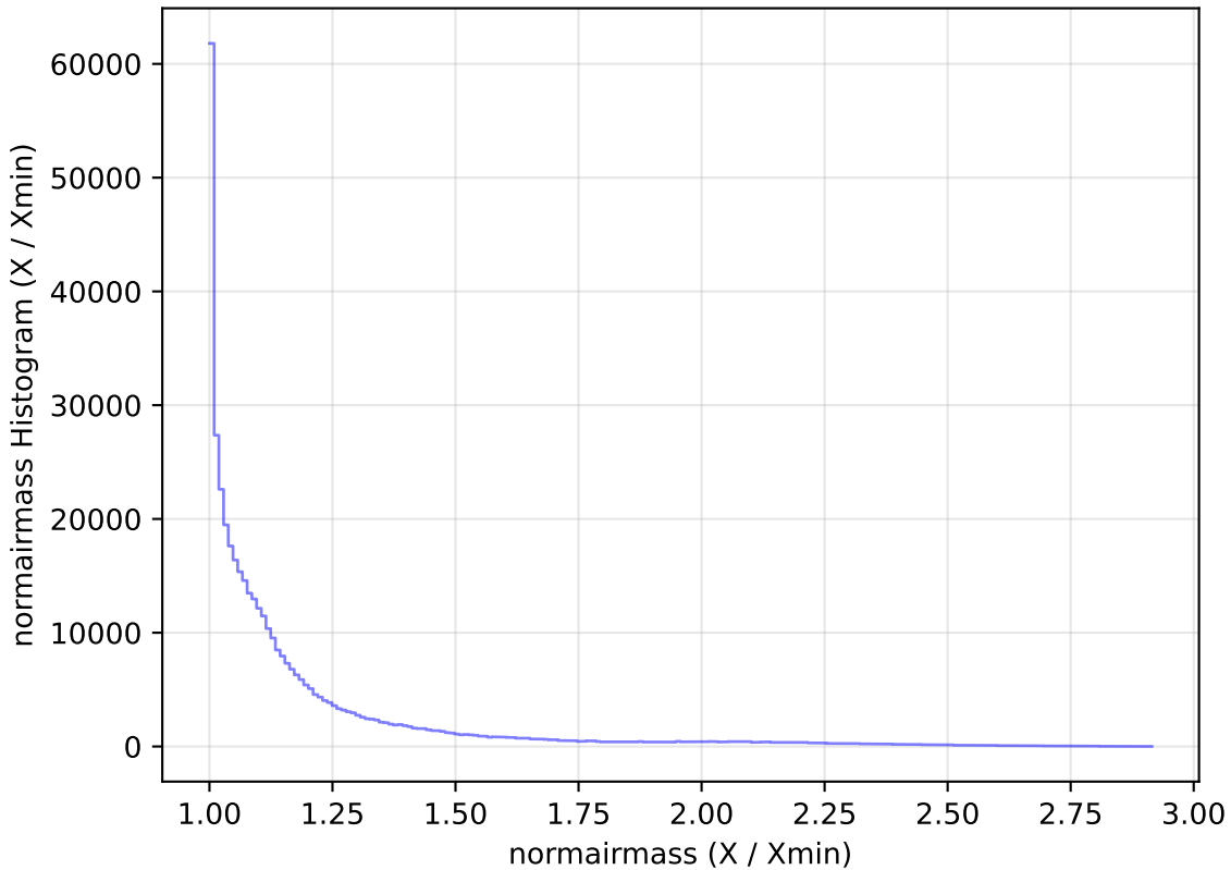
too_elab_r16_d3_giz_v3.4_10yrs WFD z band: normairmass Histogram
