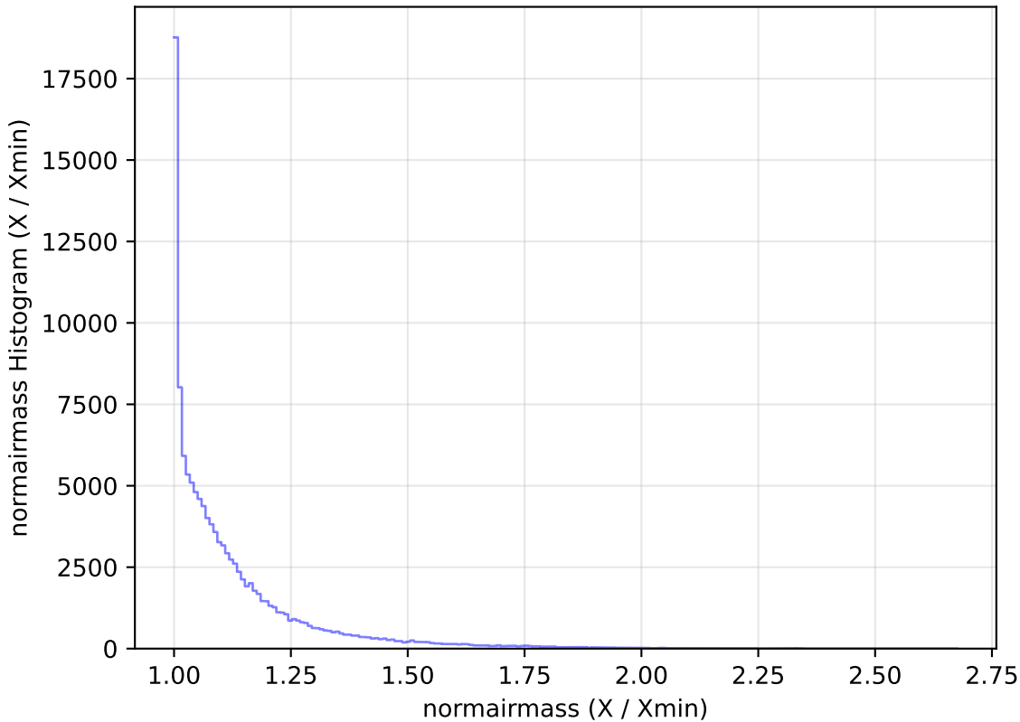
too_elab_r16_d3_giz_v3.4_10yrs WFD u band: normairmass Histogram
