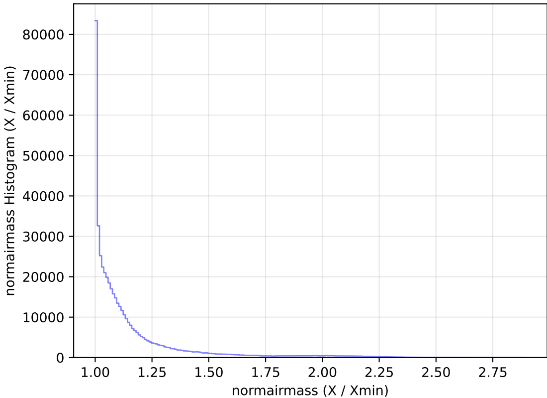
too_elab_r16_d3_giz_v3.4_10yrs WFD r band: normairmass Histogram
