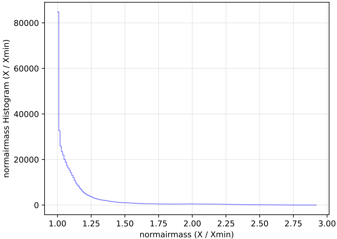
too_elab_r16_d3_giz_v3.4_10yrs WFD i band: normairmass Histogram
