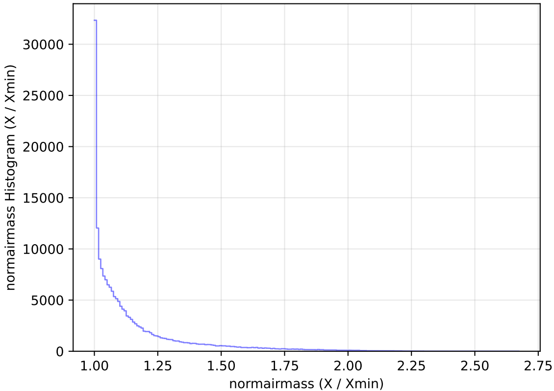
too_elab_r16_d3_giz_v3.4_10yrs WFD g band: normairmass Histogram
