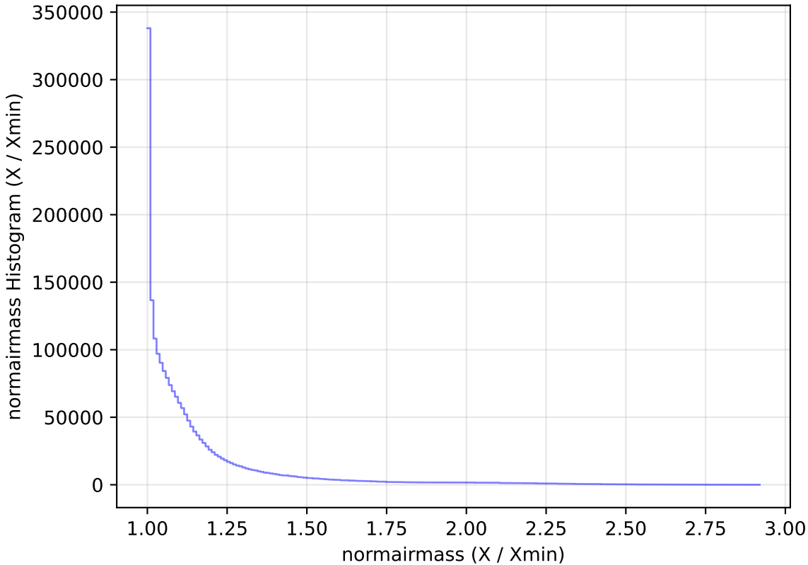
too_elab_r16_d3_giz_v3.4_10yrs WFD all bands: normairmass Histogram
