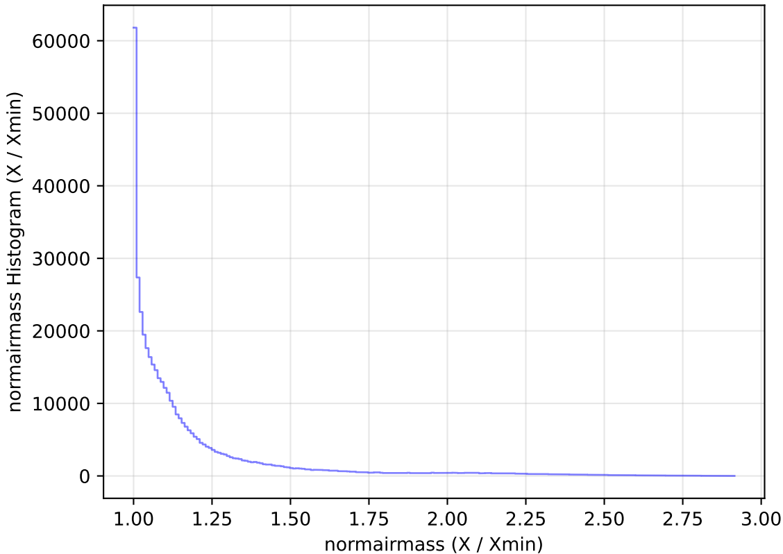
too_elab_r16_d3_giz_v3.4_10yrs All sky z band: normairmass Histogram
