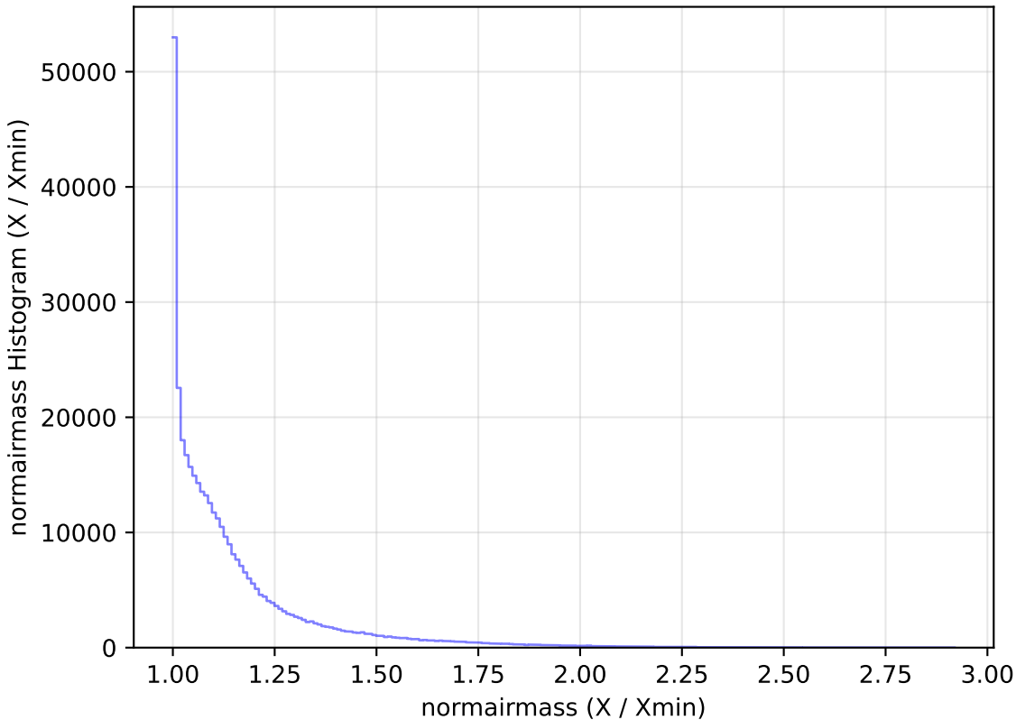
too_elab_r16_d3_giz_v3.4_10yrs All sky y band: normairmass Histogram
