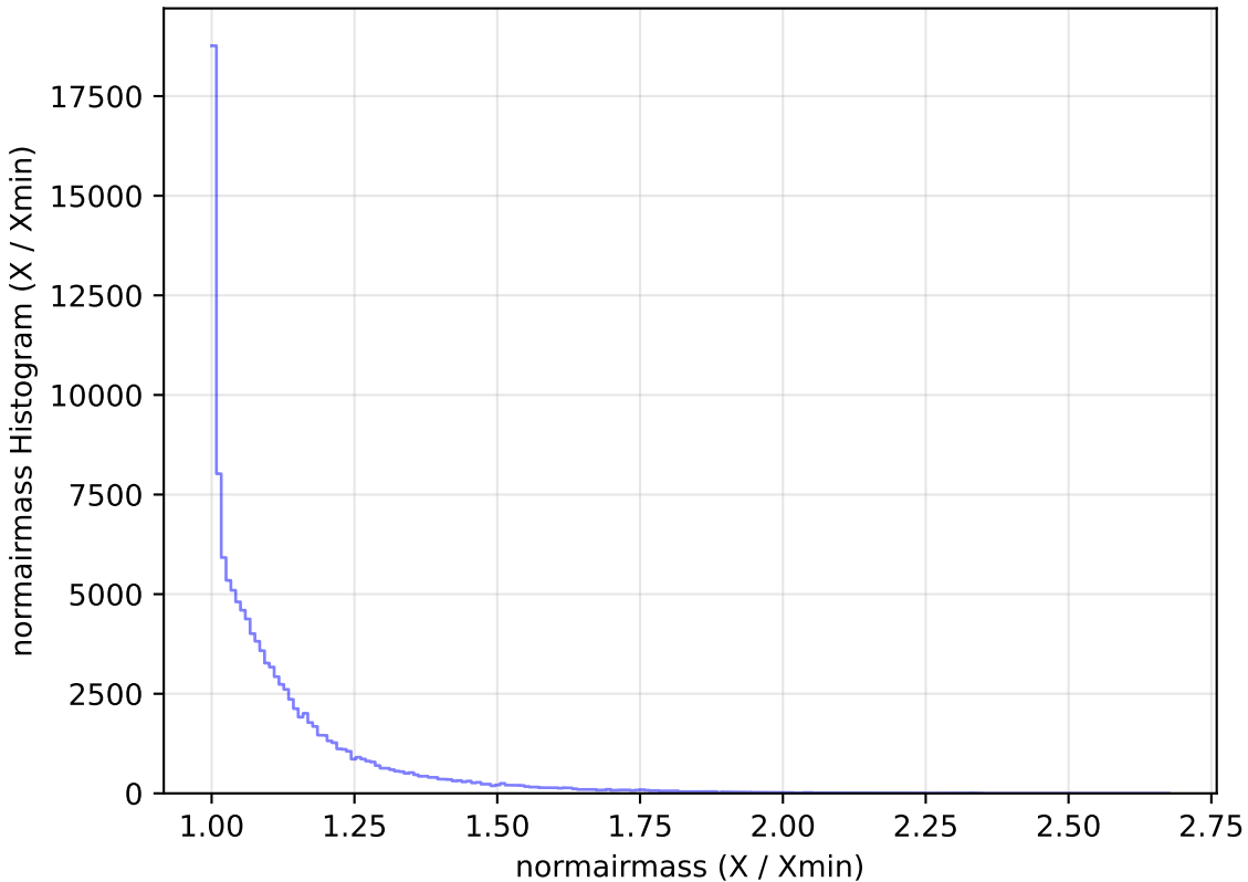
too_elab_r16_d3_giz_v3.4_10yrs All sky u band: normairmass Histogram
