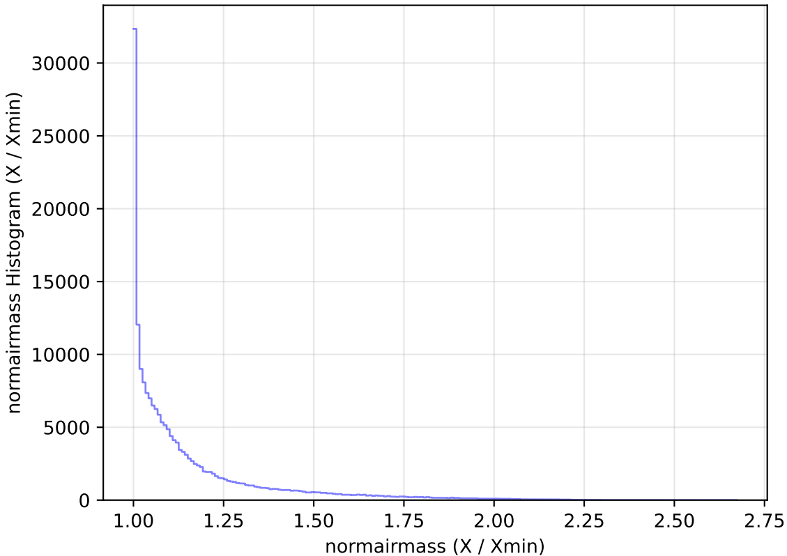
too_elab_r16_d3_giz_v3.4_10yrs All sky g band: normairmass Histogram
