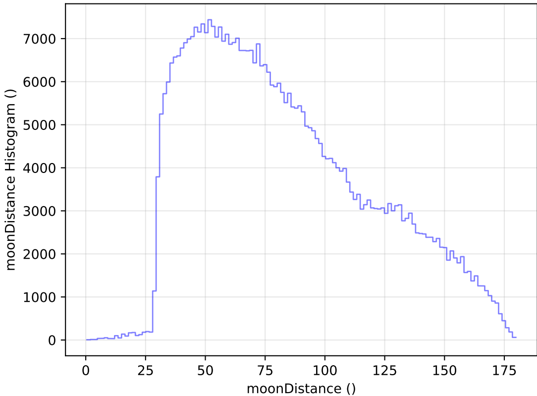
too_elab_r16_d3_giz_v3.4_10yrs WFD z band: moonDistance Histogram
