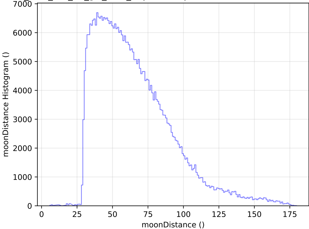
too_elab_r16_d3_giz_v3.4_10yrs WFD y band: moonDistance Histogram
