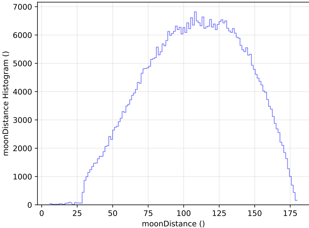
too_elab_r16_d3_giz_v3.4_10yrs WFD r band: moonDistance Histogram
