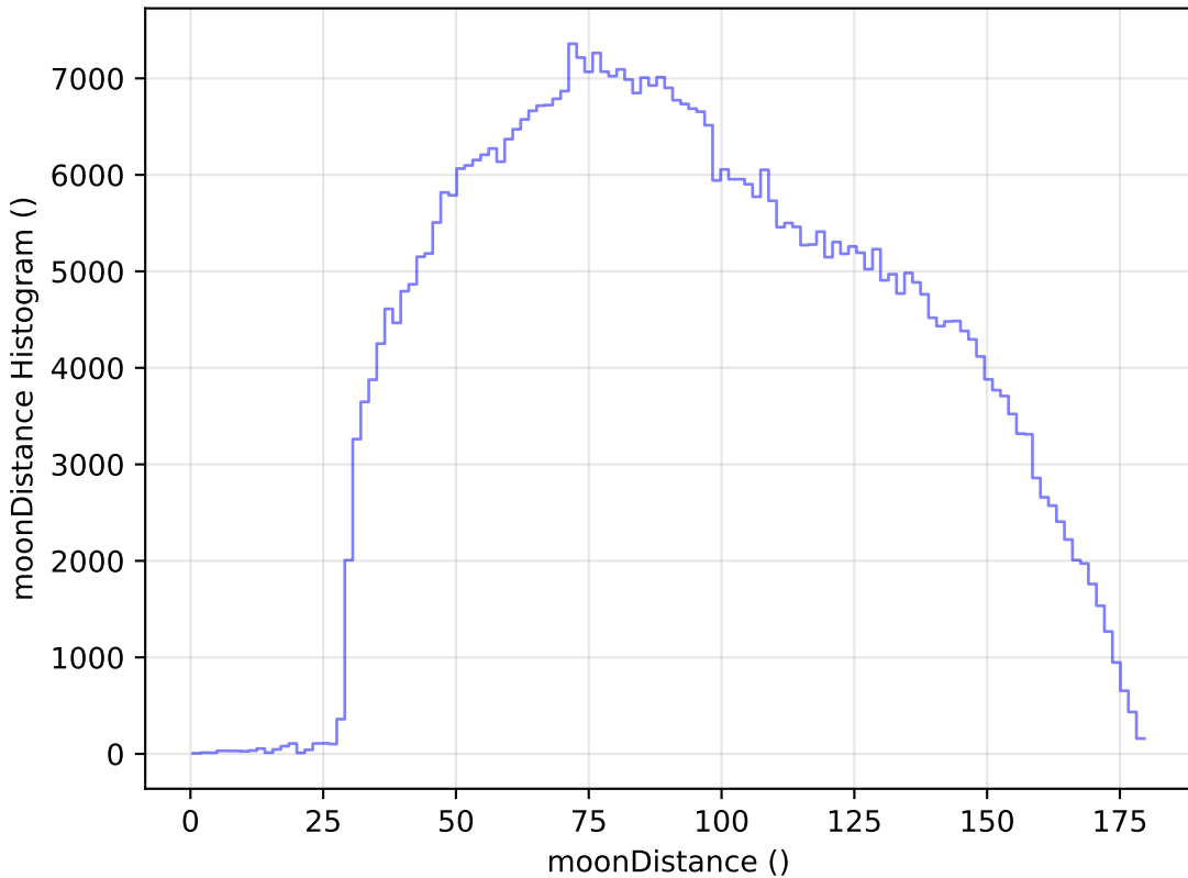
too_elab_r16_d3_giz_v3.4_10yrs WFD i band: moonDistance Histogram
