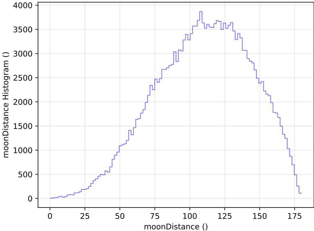
too_elab_r16_d3_giz_v3.4_10yrs WFD g band: moonDistance Histogram
