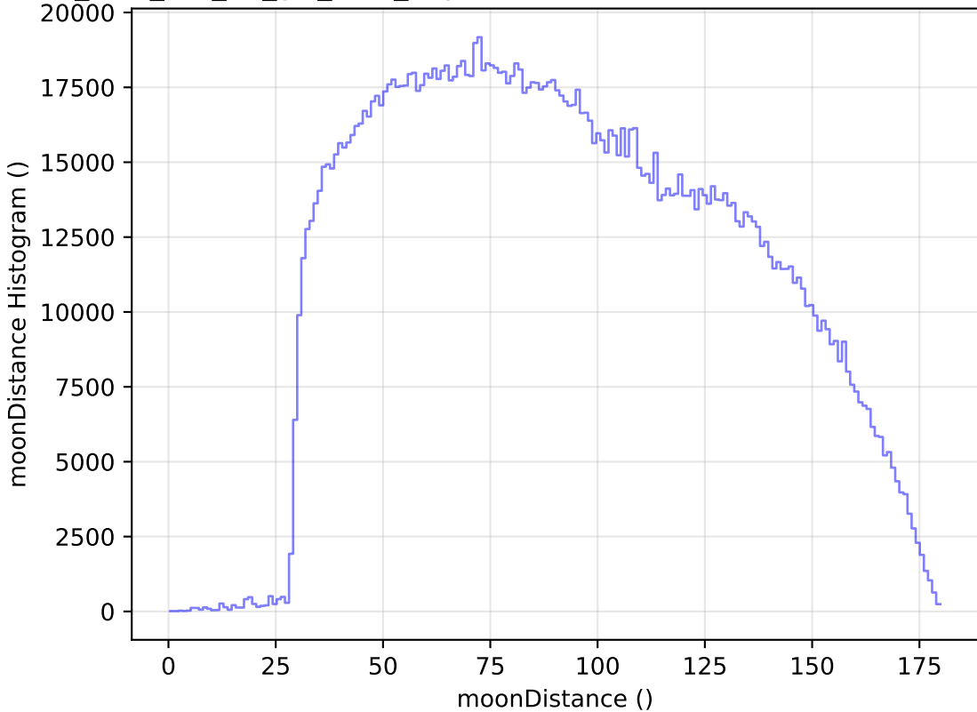
too_elab_r16_d3_giz_v3.4_10yrs WFD all bands: moonDistance Histogram
