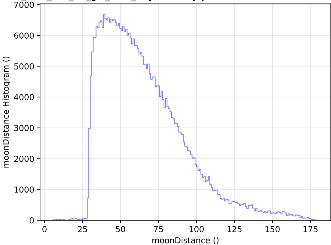
too_elab_r16_d3_giz_v3.4_10yrs All sky y band: moonDistance Histogram
