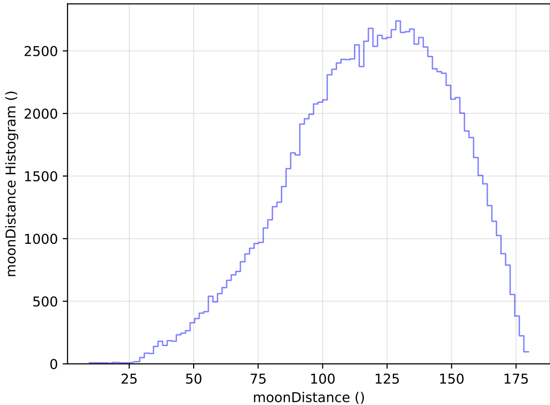
too_elab_r16_d3_giz_v3.4_10yrs All sky u band: moonDistance Histogram
