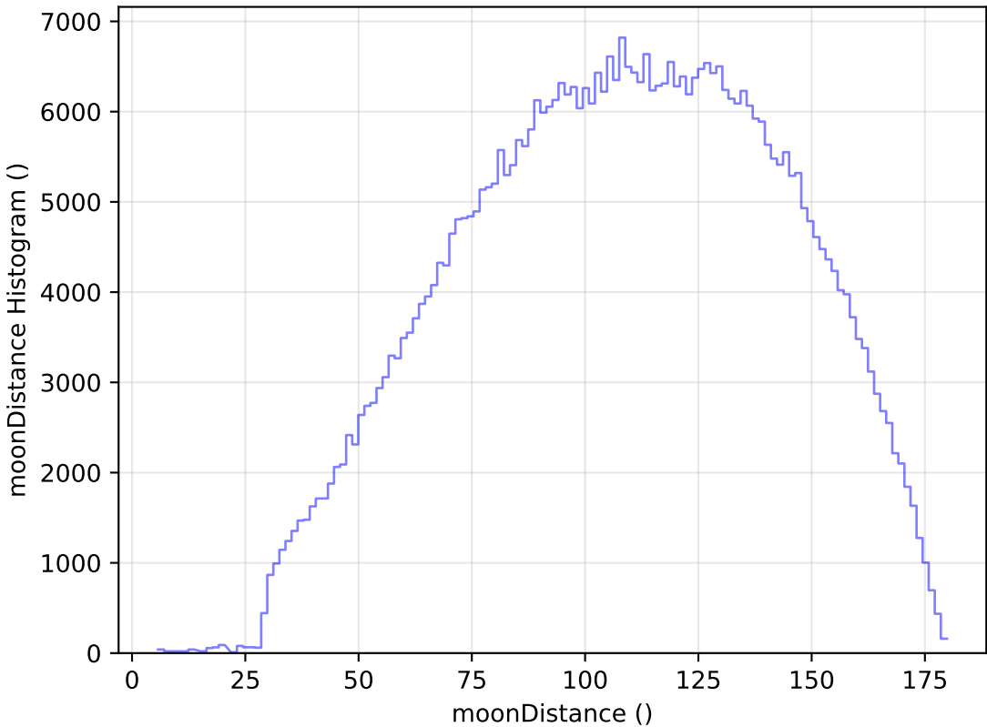
too_elab_r16_d3_giz_v3.4_10yrs All sky r band: moonDistance Histogram
