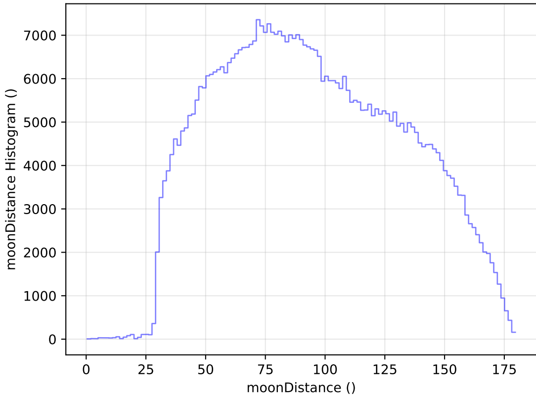
too_elab_r16_d3_giz_v3.4_10yrs All sky i band: moonDistance Histogram
