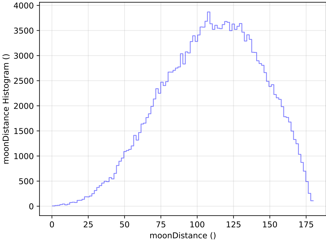
too_elab_r16_d3_giz_v3.4_10yrs All sky g band: moonDistance Histogram
