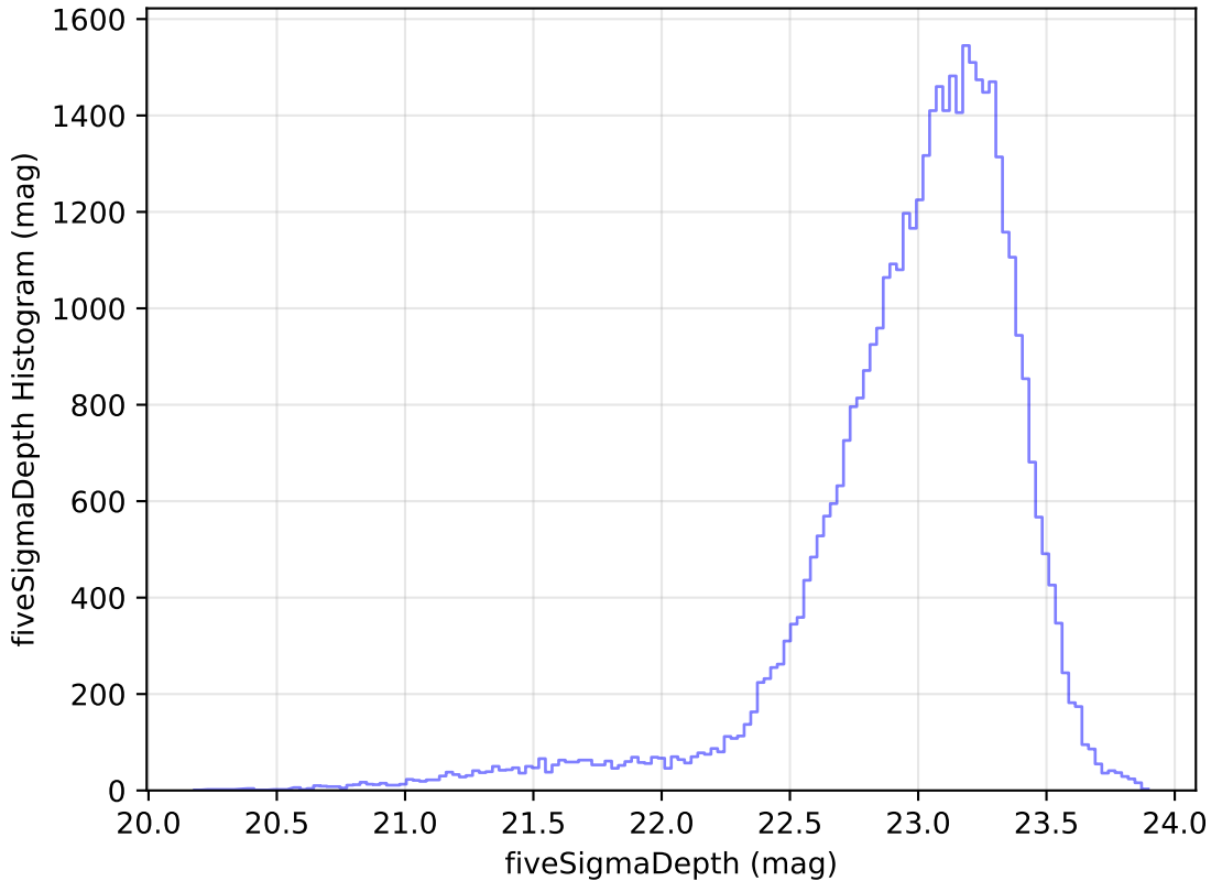
too_elab_r16_d3_giz_v3.4_10yrs Yr 1 z band: fiveSigmaDepth Histogram
