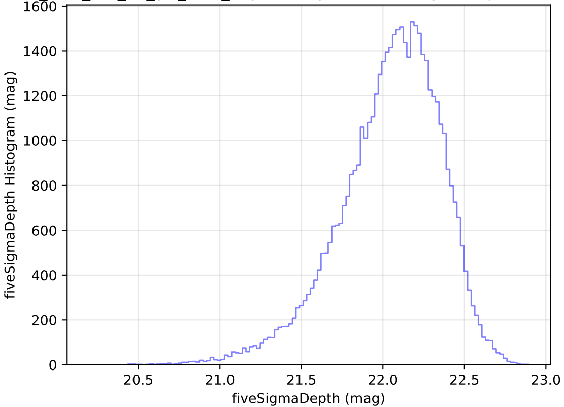
too_elab_r16_d3_giz_v3.4_10yrs Yr 1 y band: fiveSigmaDepth Histogram
