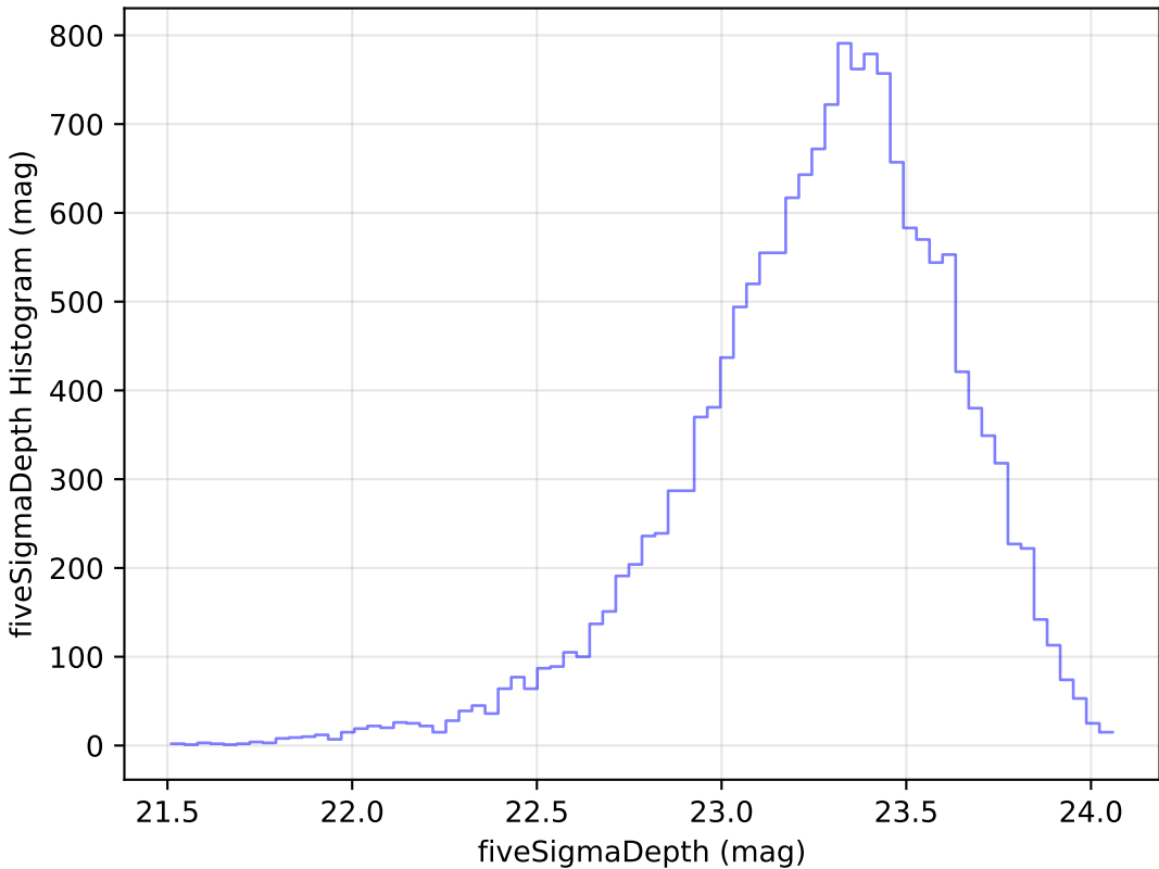
too_elab_r16_d3_giz_v3.4_10yrs Yr 1 u band: fiveSigmaDepth Histogram
