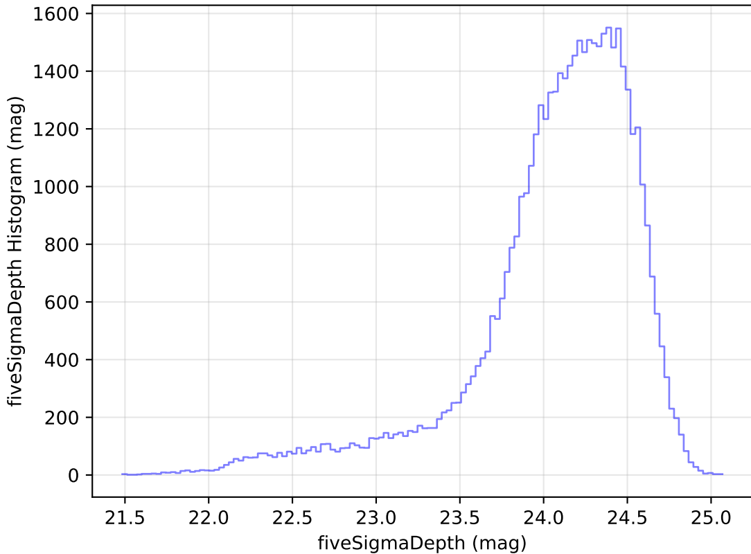
too_elab_r16_d3_giz_v3.4_10yrs Yr 1 r band: fiveSigmaDepth Histogram
