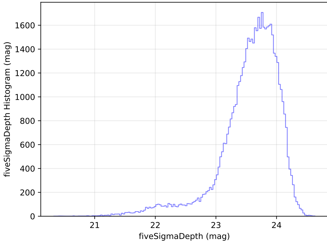
too_elab_r16_d3_giz_v3.4_10yrs Yr 1 i band: fiveSigmaDepth Histogram
