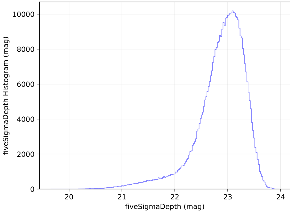
too_elab_r16_d3_giz_v3.4_10yrs WFD z band: fiveSigmaDepth Histogram
