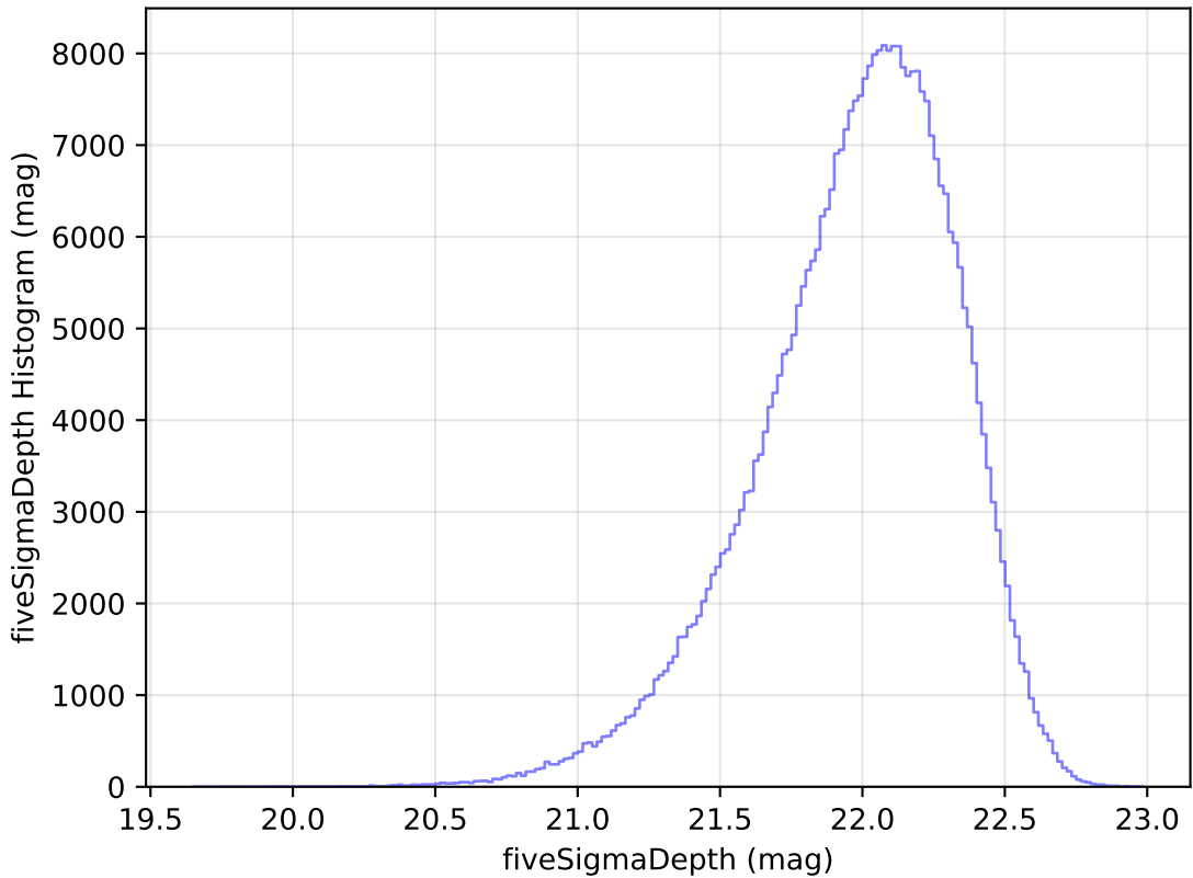
too_elab_r16_d3_giz_v3.4_10yrs WFD y band: fiveSigmaDepth Histogram
