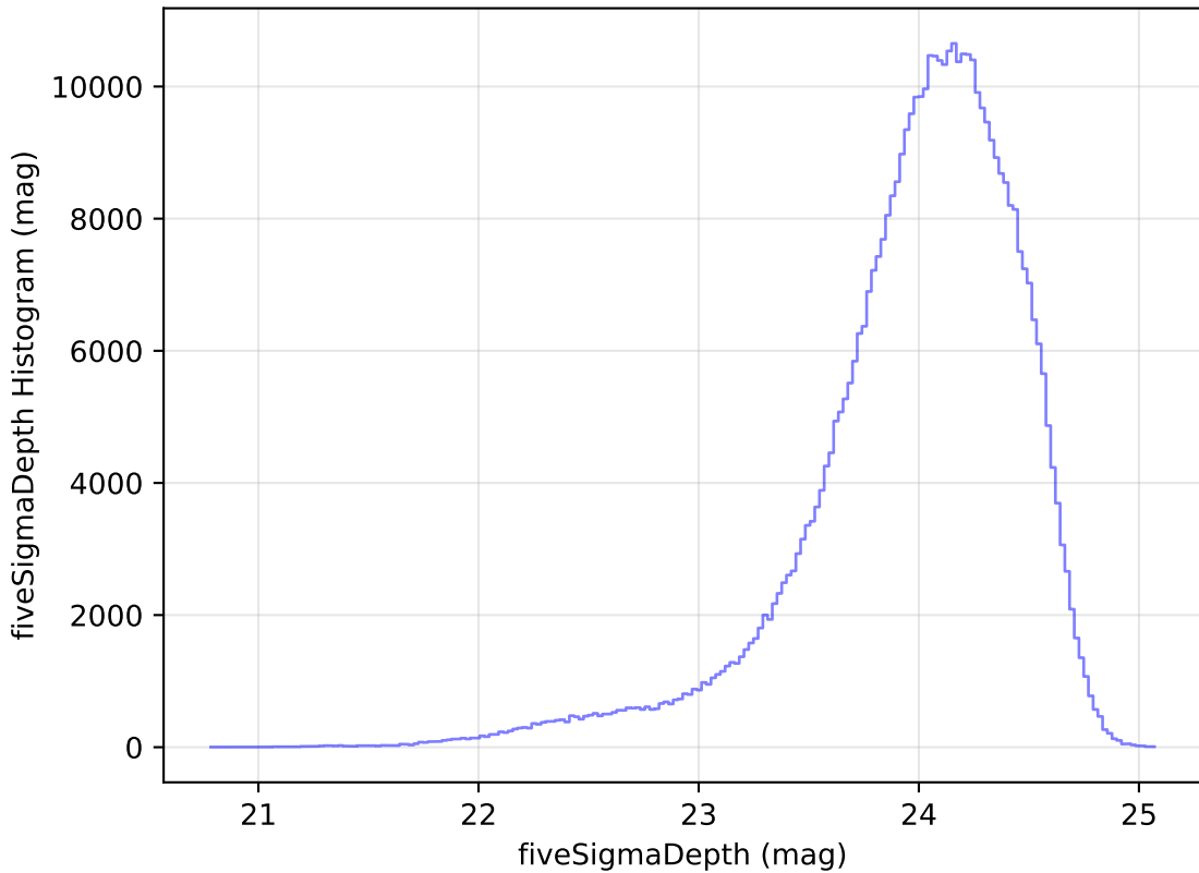
too_elab_r16_d3_giz_v3.4_10yrs WFD r band: fiveSigmaDepth Histogram
