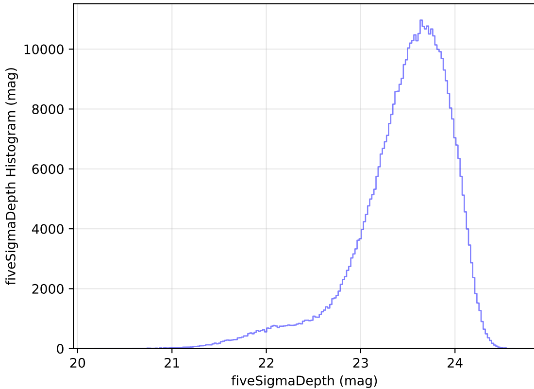
too_elab_r16_d3_giz_v3.4_10yrs WFD i band: fiveSigmaDepth Histogram
