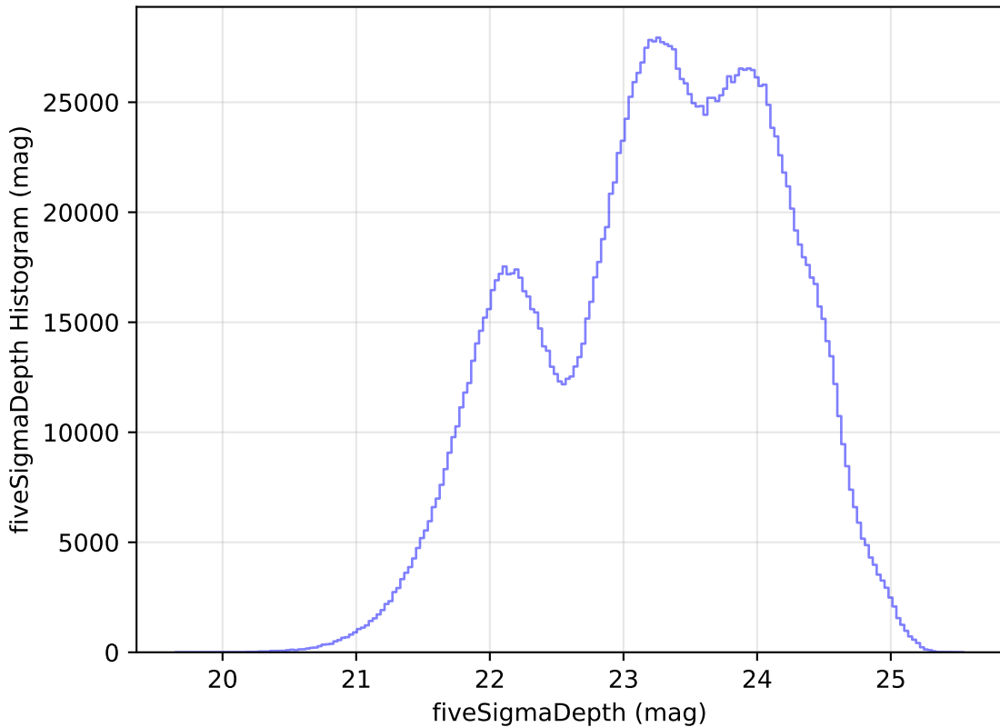
too_elab_r16_d3_giz_v3.4_10yrs WFD all bands: fiveSigmaDepth Histogram
