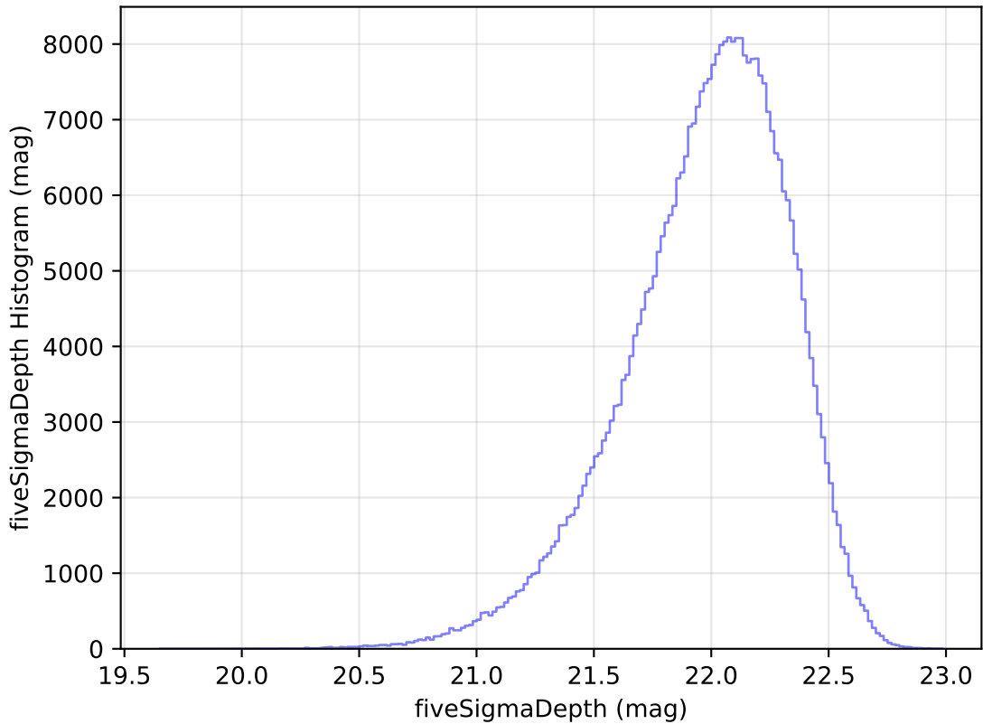
too_elab_r16_d3_giz_v3.4_10yrs All sky y band: fiveSigmaDepth Histogram
