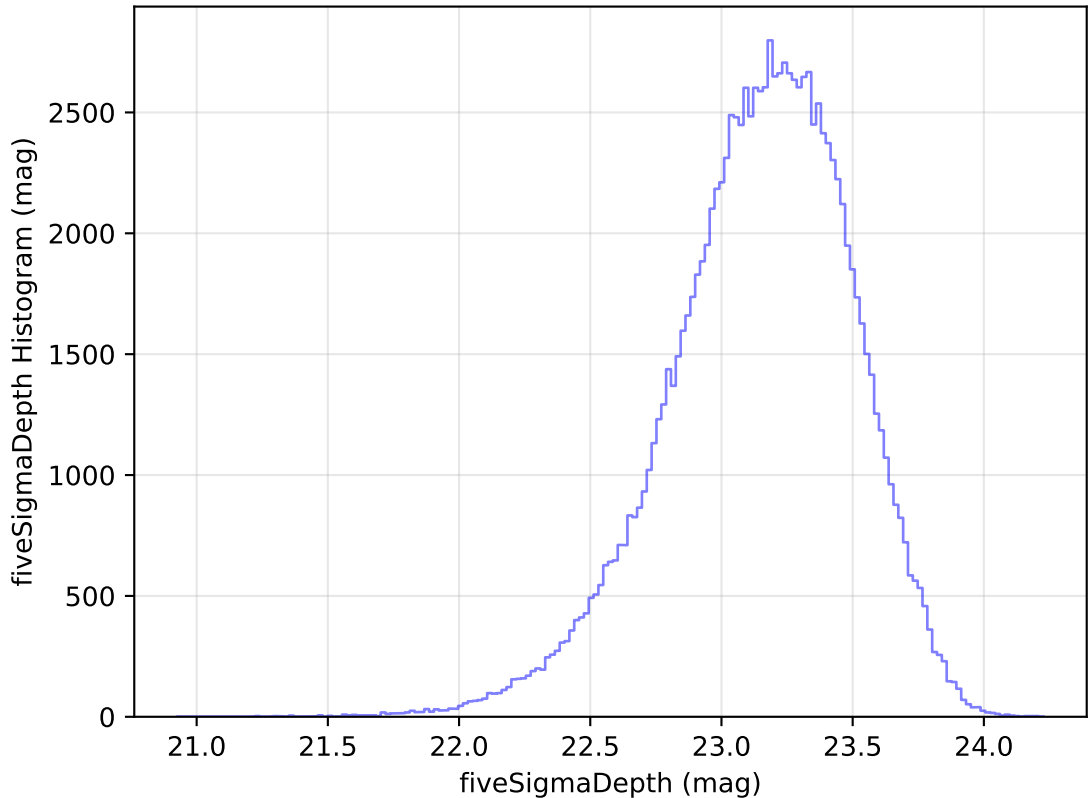
too_elab_r16_d3_giz_v3.4_10yrs All sky u band: fiveSigmaDepth Histogram
