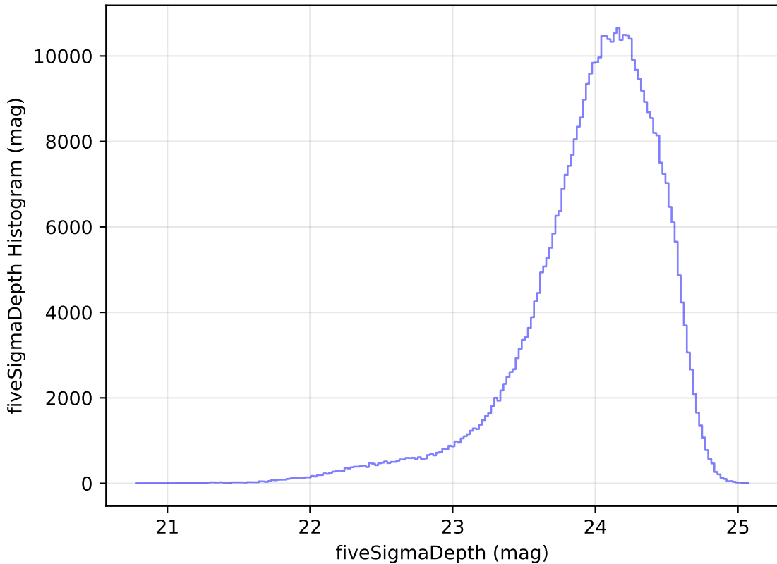
too_elab_r16_d3_giz_v3.4_10yrs All sky r band: fiveSigmaDepth Histogram
