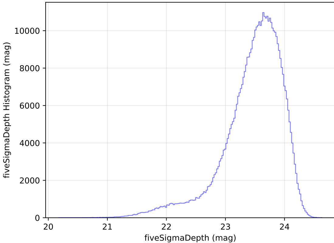
too_elab_r16_d3_giz_v3.4_10yrs All sky i band: fiveSigmaDepth Histogram
