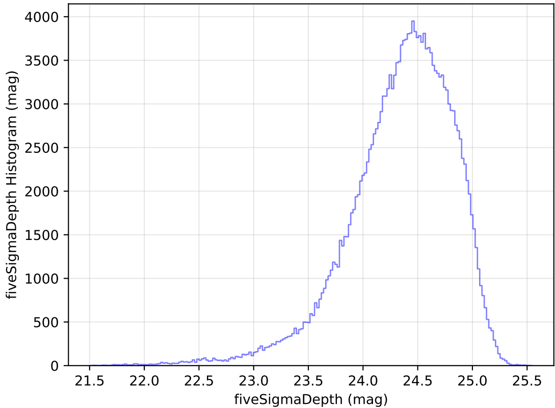
too_elab_r16_d3_giz_v3.4_10yrs All sky g band: fiveSigmaDepth Histogram
