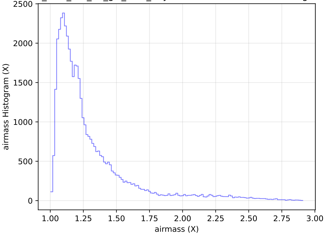
too_elab_r16_d3_giz_v3.4_10yrs Yr 1 z band: airmass Histogram
