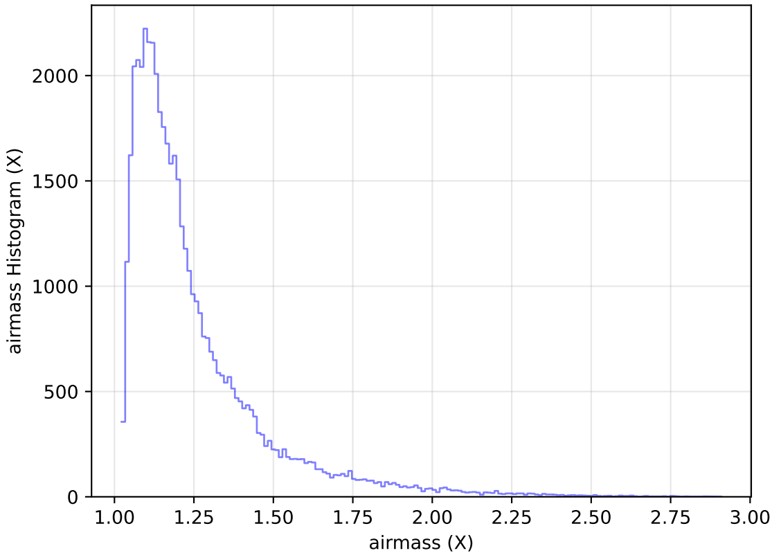
too_elab_r16_d3_giz_v3.4_10yrs Yr 1 y band: airmass Histogram
