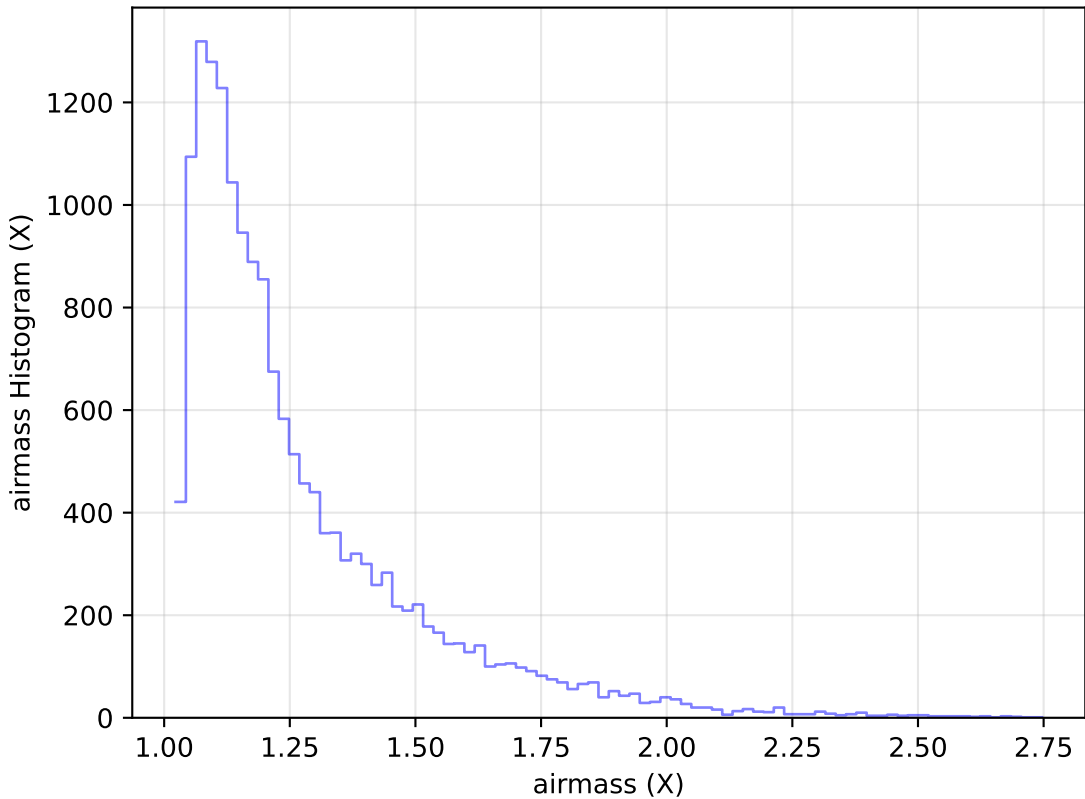
too_elab_r16_d3_giz_v3.4_10yrs Yr 1 u band: airmass Histogram
