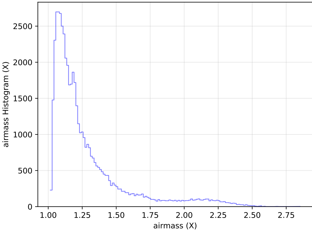
too_elab_r16_d3_giz_v3.4_10yrs Yr 1 r band: airmass Histogram
