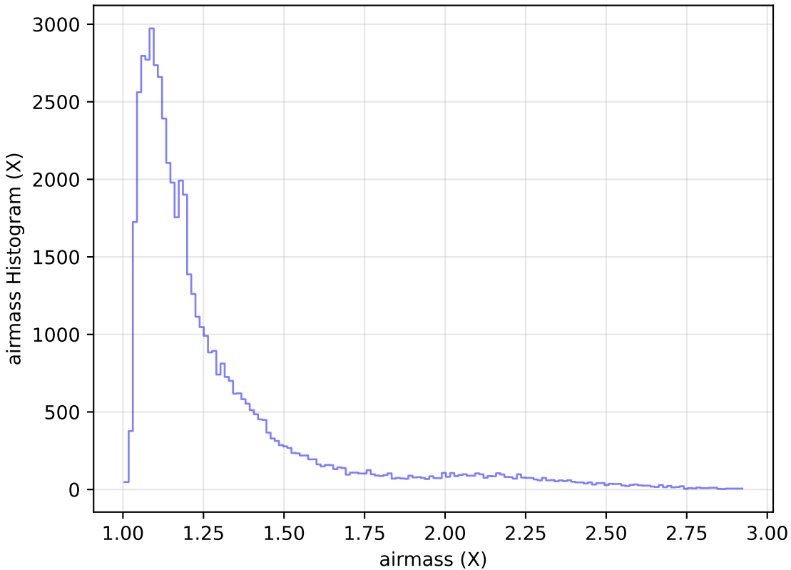
too_elab_r16_d3_giz_v3.4_10yrs Yr 1 i band: airmass Histogram
