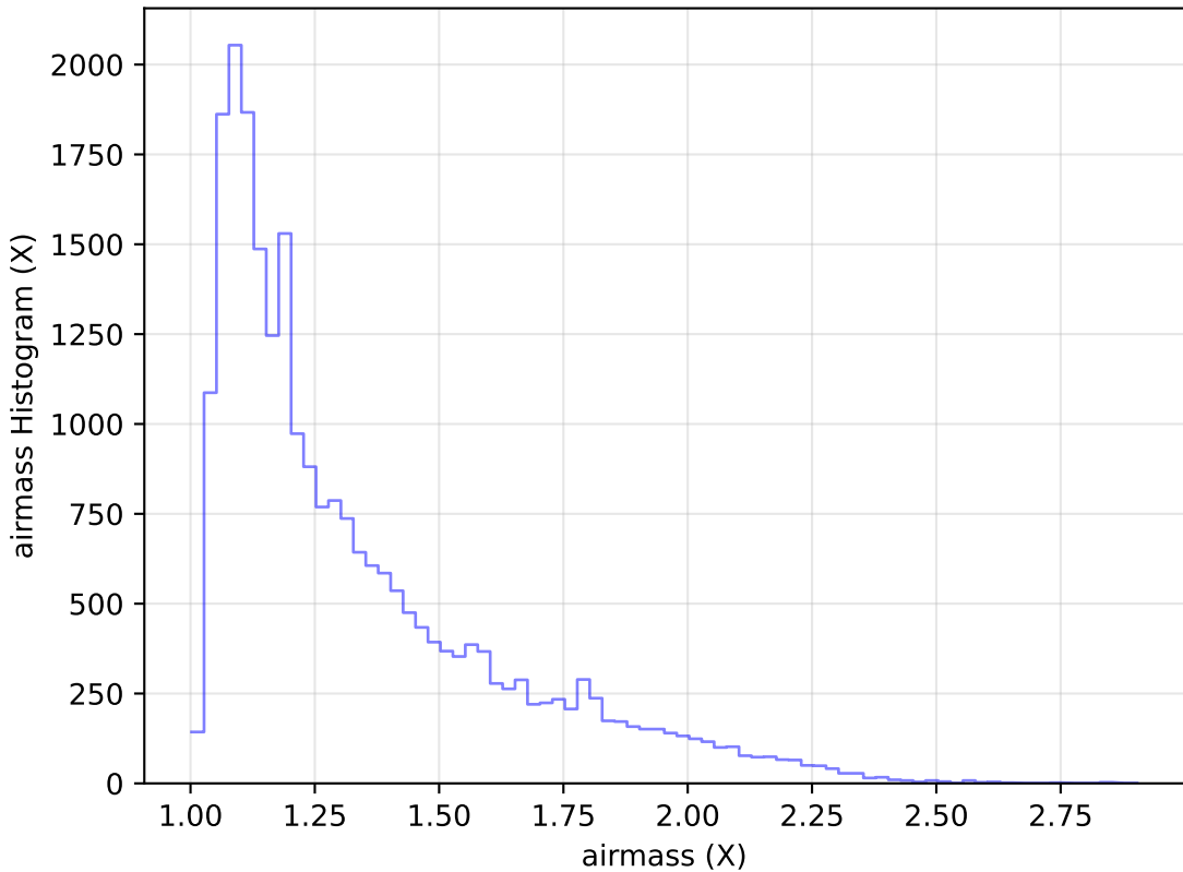
too_elab_r16_d3_giz_v3.4_10yrs Yr 1 g band: airmass Histogram
