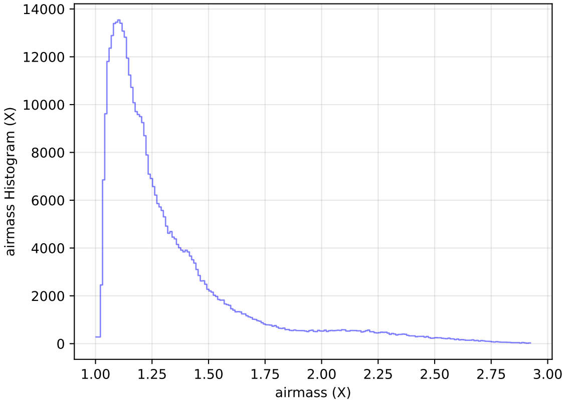
too_elab_r16_d3_giz_v3.4_10yrs WFD z band: airmass Histogram
