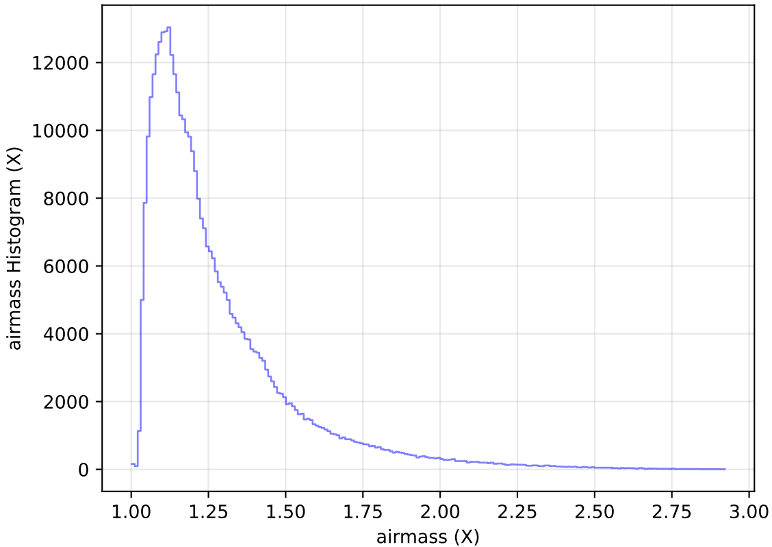
too_elab_r16_d3_giz_v3.4_10yrs WFD y band: airmass Histogram
