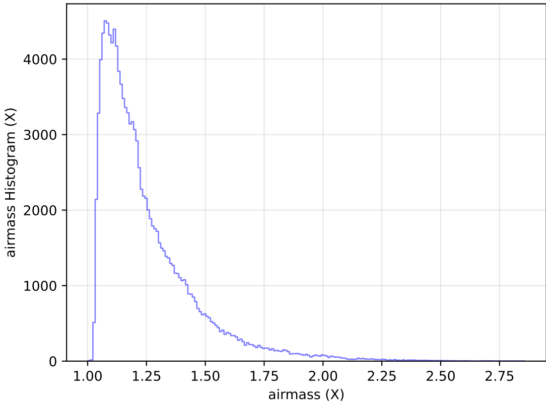
too_elab_r16_d3_giz_v3.4_10yrs WFD u band: airmass Histogram
