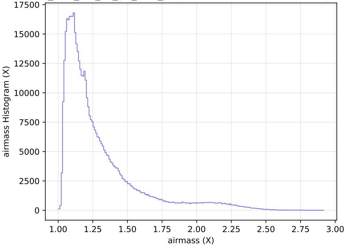
too_elab_r16_d3_giz_v3.4_10yrs WFD r band: airmass Histogram
