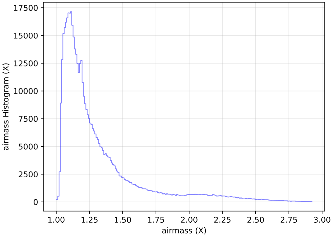
too_elab_r16_d3_giz_v3.4_10yrs WFD i band: airmass Histogram
