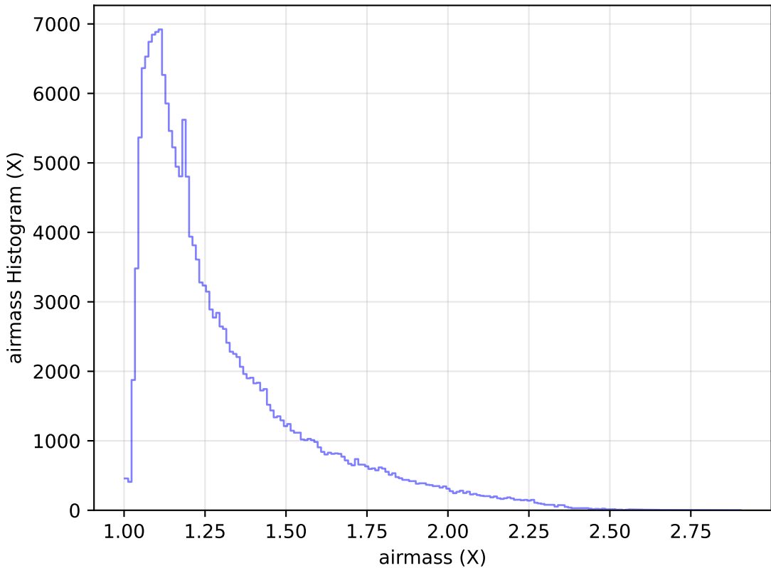
too_elab_r16_d3_giz_v3.4_10yrs WFD g band: airmass Histogram
