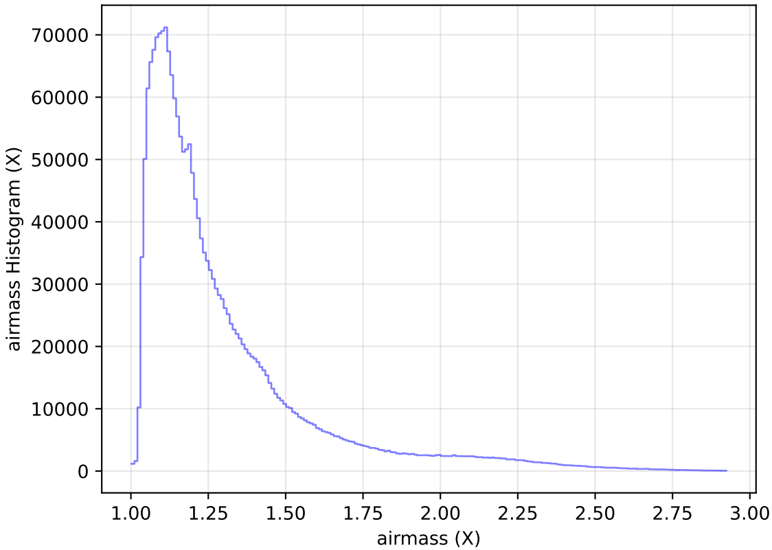
too_elab_r16_d3_giz_v3.4_10yrs WFD all bands: airmass Histogram
