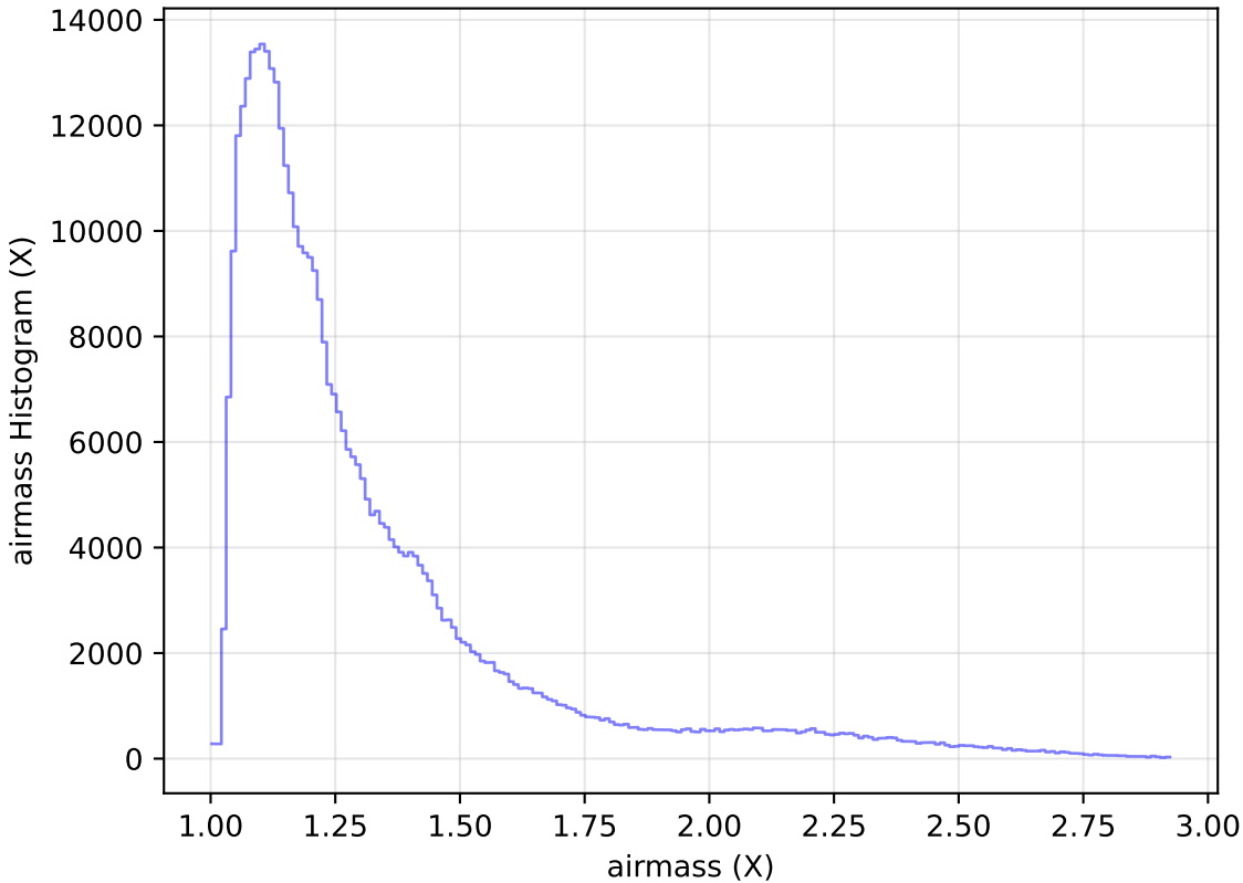
too_elab_r16_d3_giz_v3.4_10yrs All sky z band: airmass Histogram
